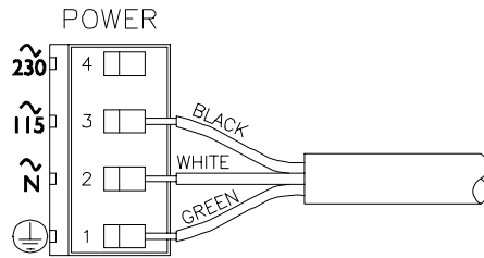
FIGURE 2-15 Connecting 115 Volt Single Phase to Analyzers with "A" or No Letter Prefix Serial Number
