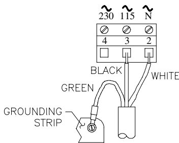
FIGURE 2-12 Connecting 115 Volt Single Phase to Analyzers with "B" Prefix Serial Number
