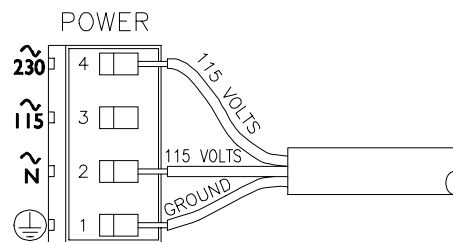
FIGURE 2-17 Connecting 230 Volt Split Phase to Analyzers with "A" or No Letter Prefix Serial Number
